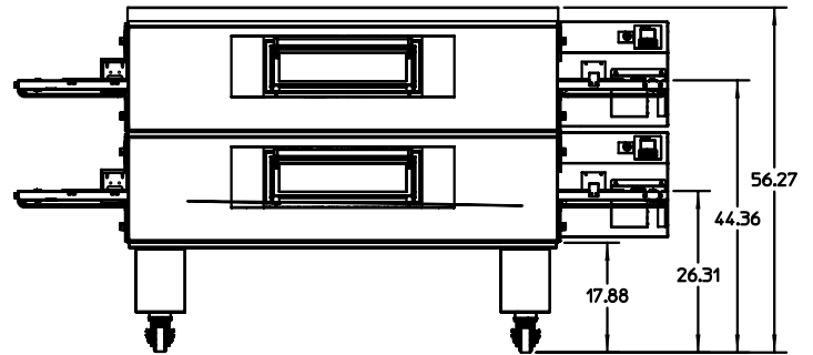
X70 Front View – Gas, Double Unit
