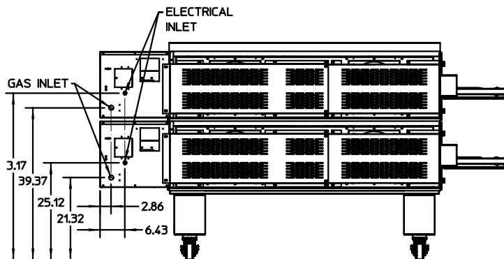
X70 Back View – Gas, Double Unit
