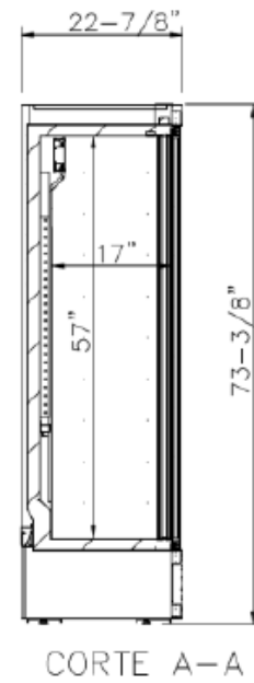
RIGHT VIEW
