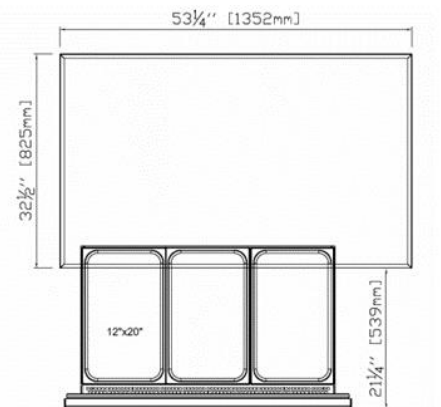
RIGHT VIEW
