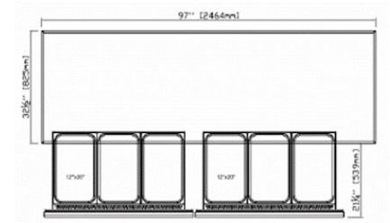
RIGHT VIEW
