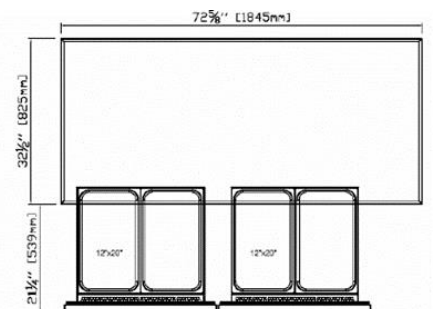
RIGHT VIEW
