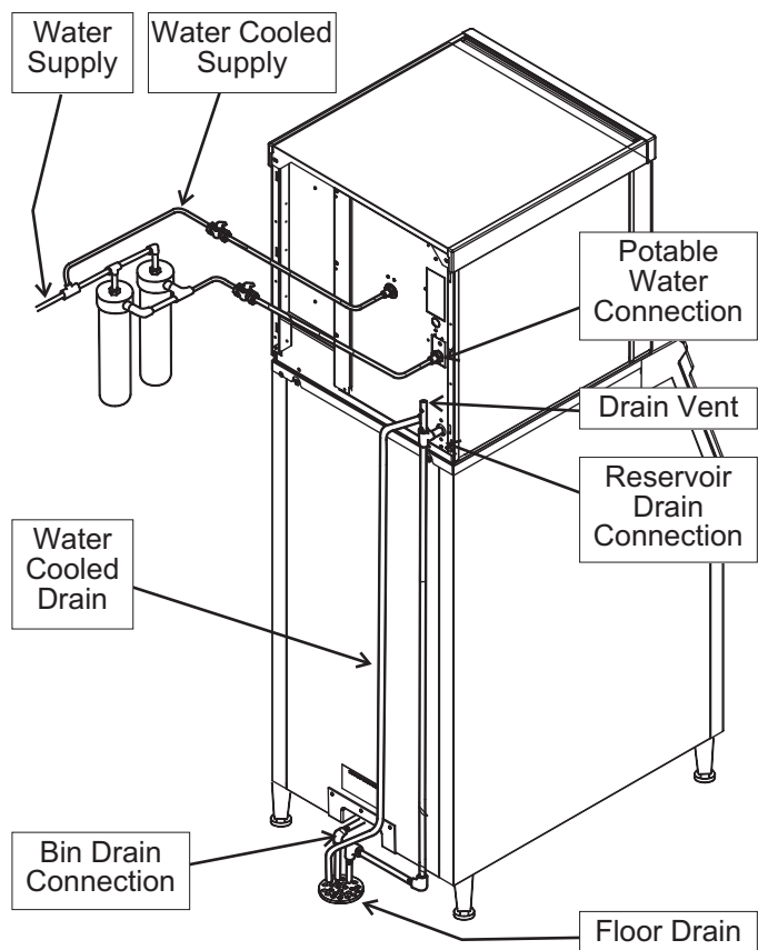
Plumbing Connections
