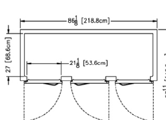
Plan - R/AHF332W
