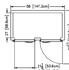
Plan - R/AHF232W
