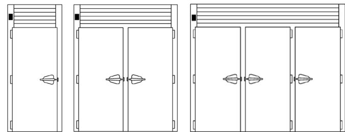
Elevation - R/AIH132LP
