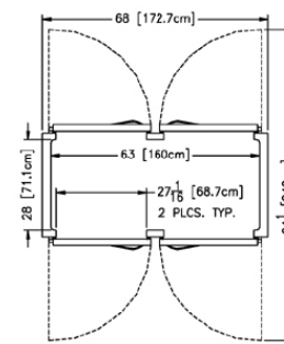
Plan - R/AIH232LP
