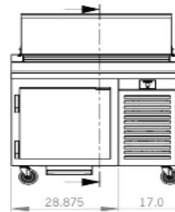
Elevation View
