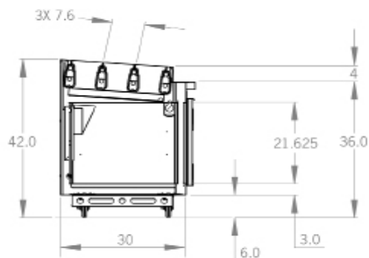
3-Row Section View
