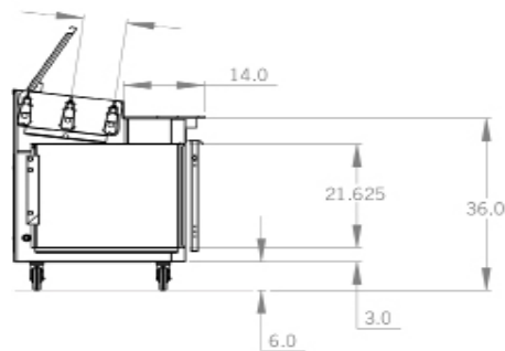
Section View
