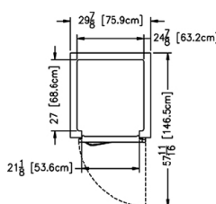
Plan - R/ACV132WUT
