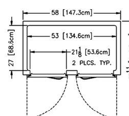
Plan - R/ACV232WUT
