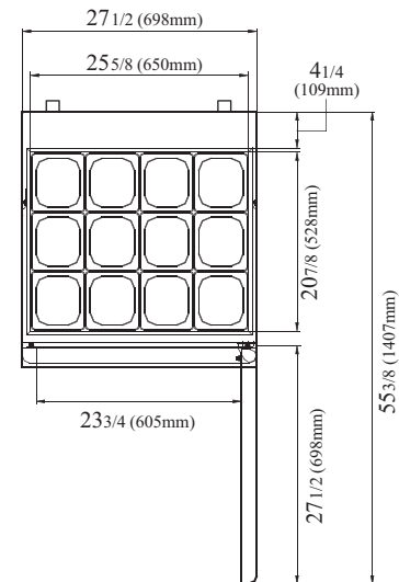
PLAN VIEW
