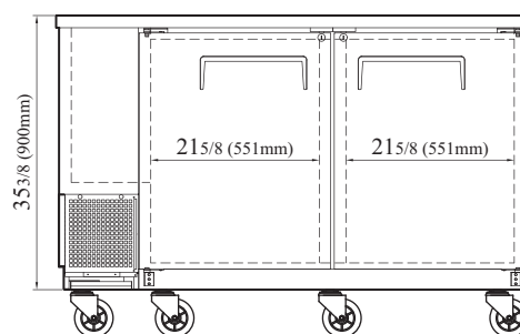
TBB-24-60SB-N6 FRONT VIEW
