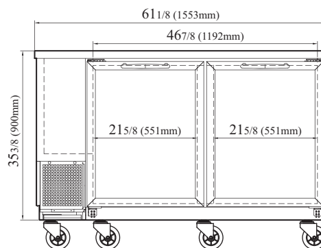
TBB-24-60SG-N FRONT VIEW
