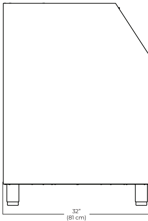
SIDE VIEW
