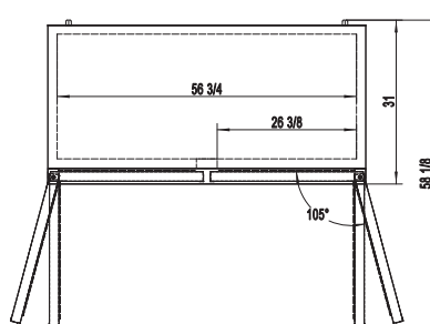
Rear grate
