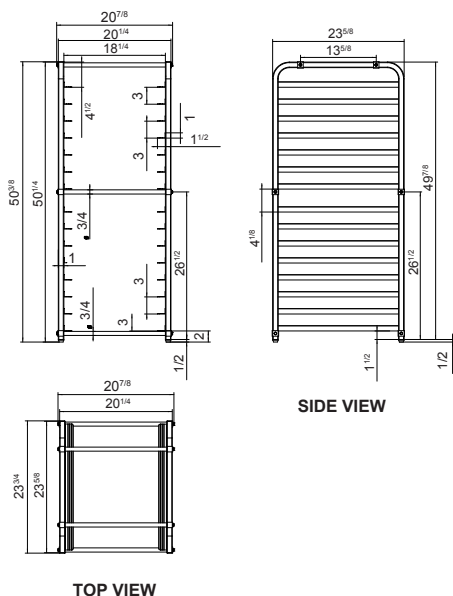
SPA15K1824X
