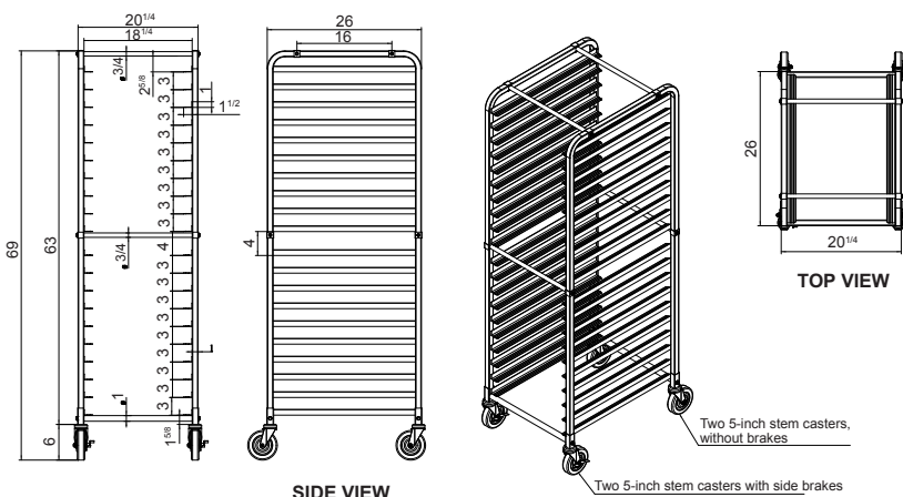
SPA20K1826
